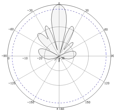
Horizontal Pattern
