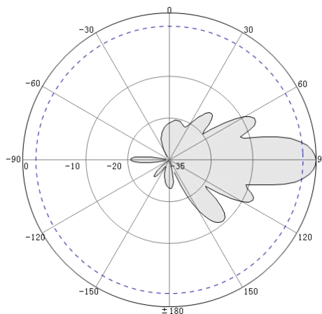
Vertical Pattern
