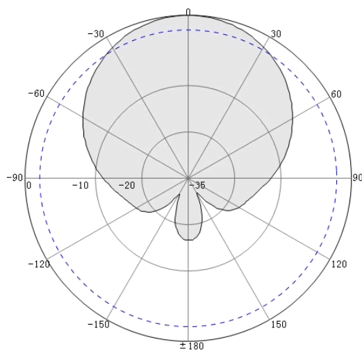
Horizontal Pattern
