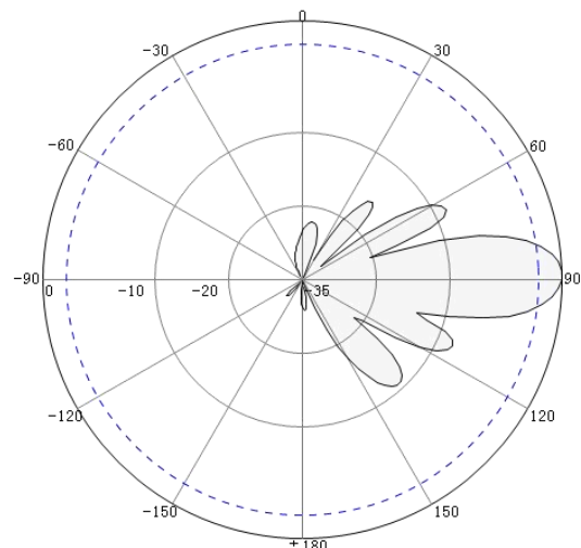
Vertical Pattern
